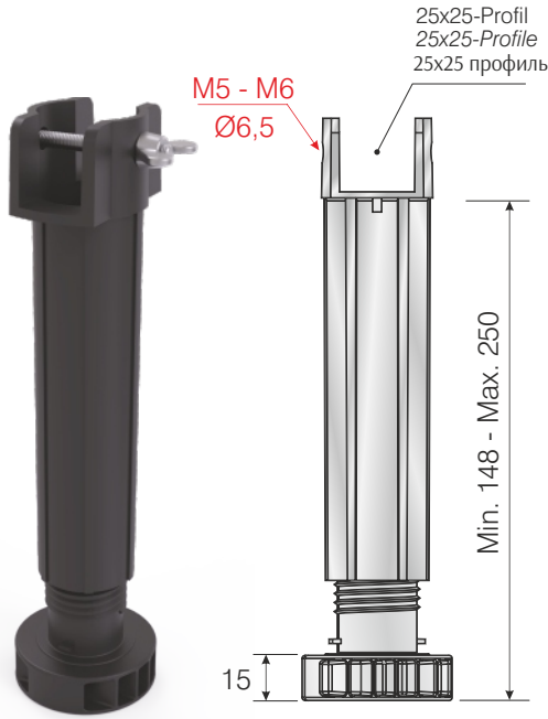
104-01-38 25x25-Profile
