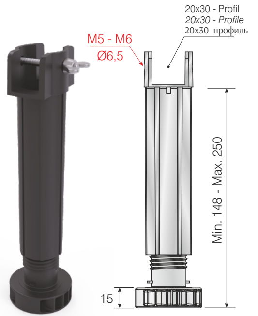
104-01-43 20x30-Profile
