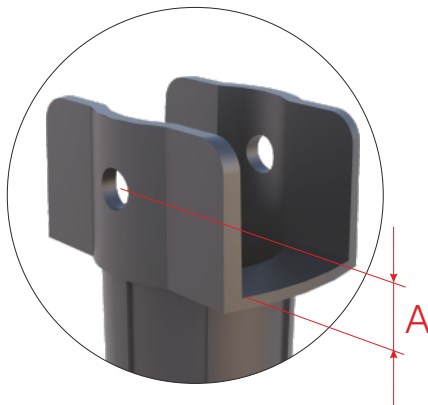
104-01-38 A=12,5mm
