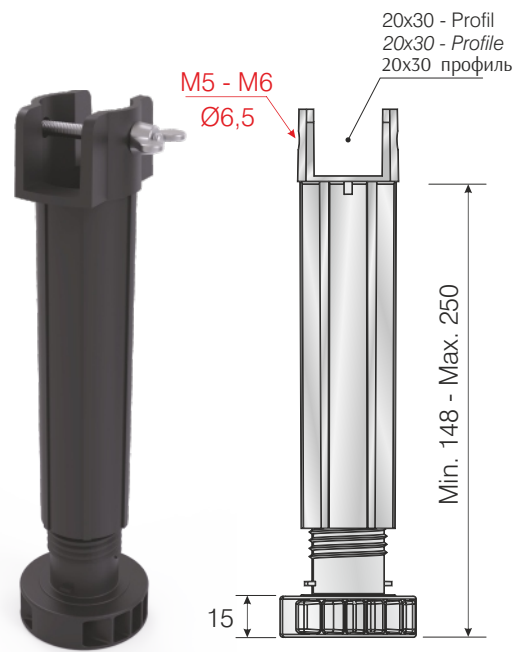
104-01-43 20x30-Profile
